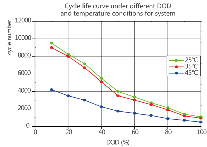
Cycle Life Curves
